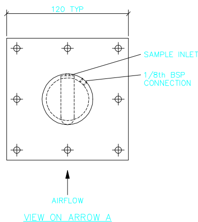
DIAGRAM SHOWING SCDP MOUNTED IN A DUCT
