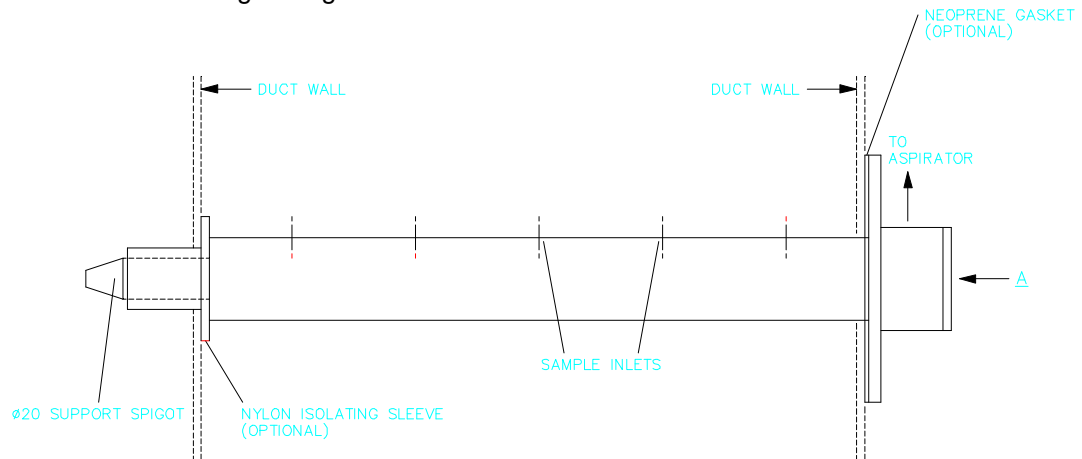
DIAGRAM SHOWING SCDP MOUNTED IN A DUCT
